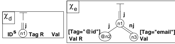
Figure 2: Sample XAMs \chi_d and \chi_e .
