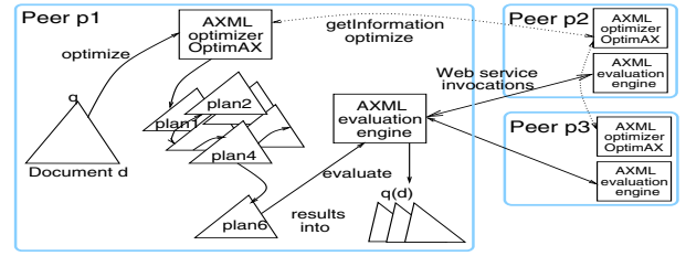
Fig. 1. AXML optimization process.
