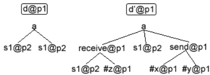
Fig. 3. Factorization example.
