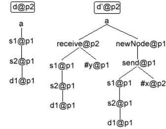
Fig. 2. Delegation example.
